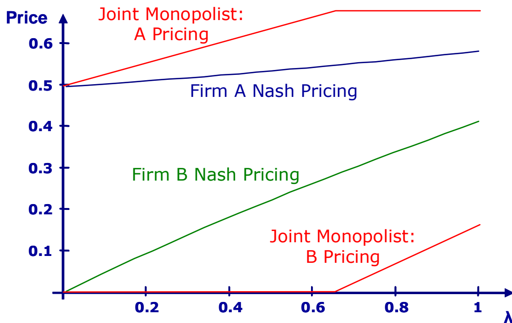
Figure 4: Nash Pricing and Joint A & B Monopolist Pricing.
